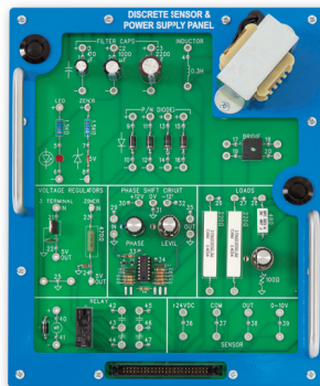
Discrete Sensor & Power Supply Panel
