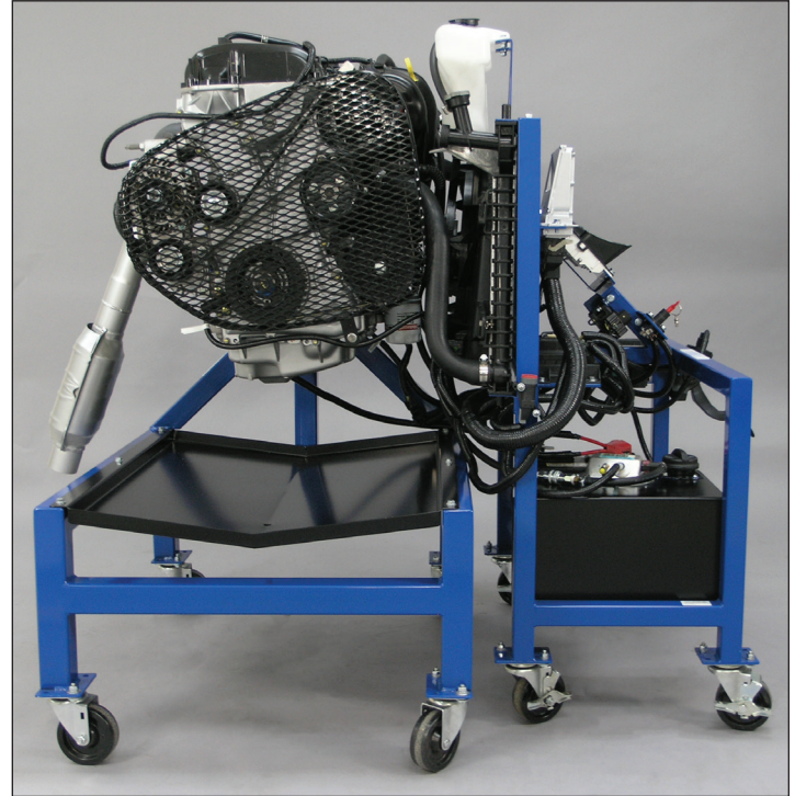
Engine Repair Trainer (model 90) connected to Engine Start Cart (model 91)
